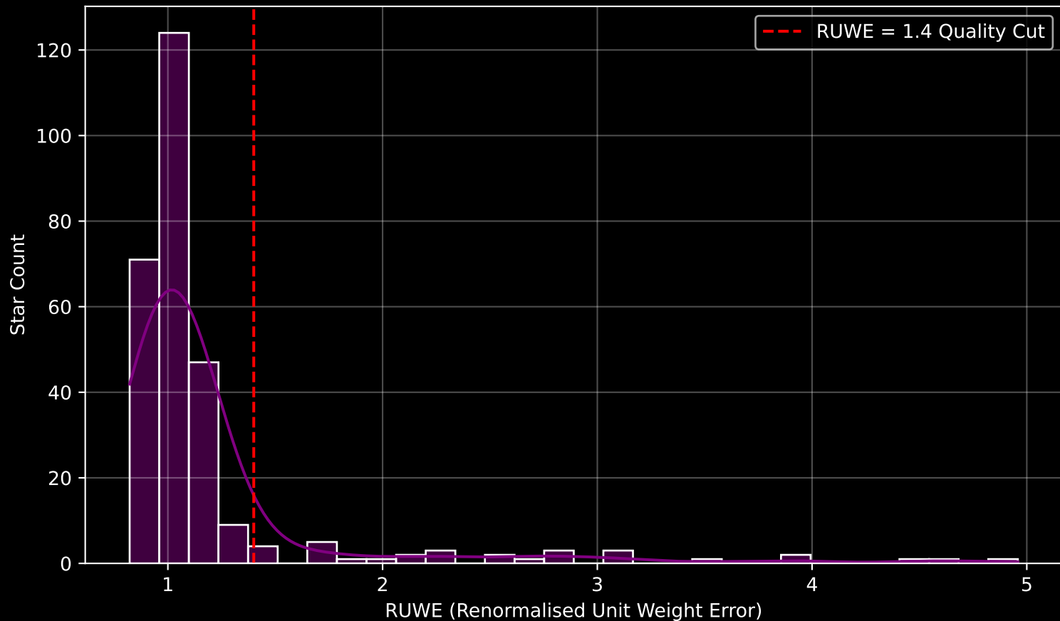
GALAH DR4 Field [281] RUWE Distribution (n= 282)
