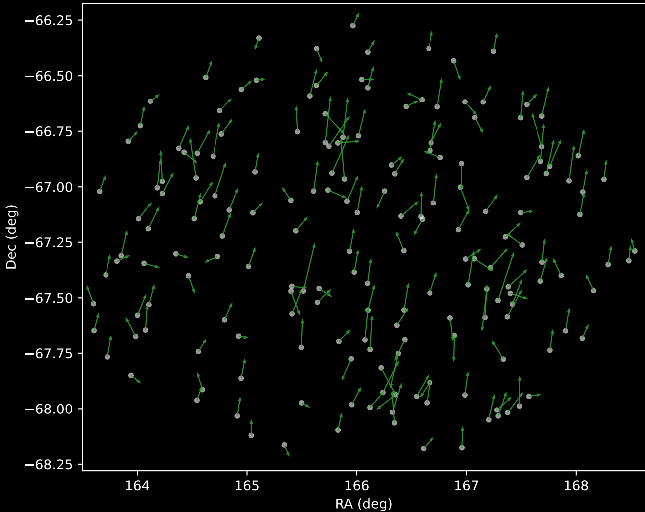
GALAH DR4 Cluster 4 Proper Motion Vectors (n=179)
