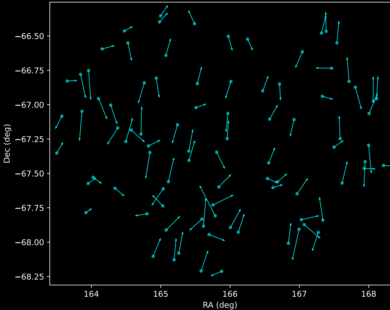
GALAH DR4 Noise Stream Proper Motion Vectors (n=89)
